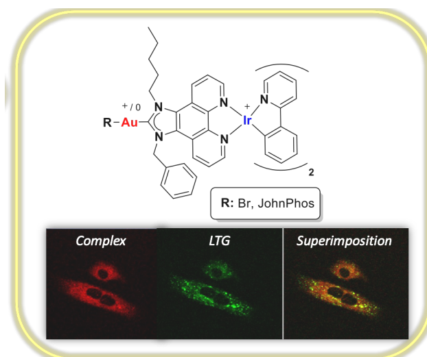
Figure1. Schematic representation of the heterometallic photosensitizers.
