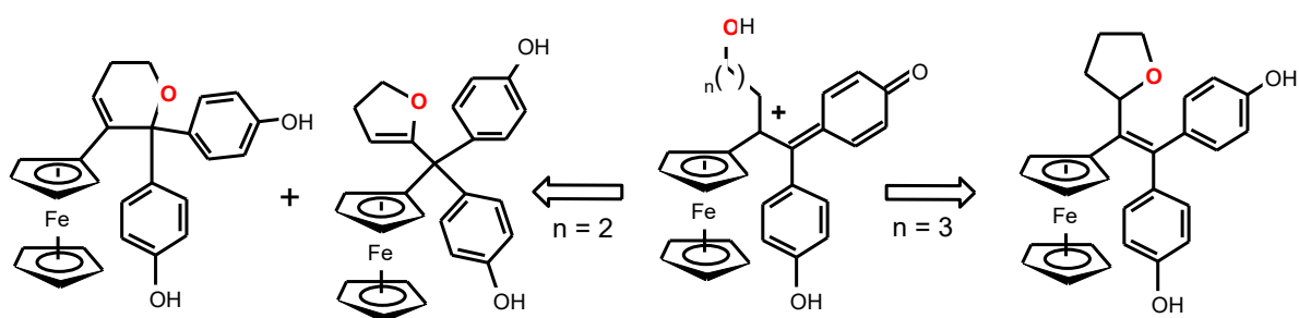
Figure 1. Molecular rearrangements of hydroxyalkyl-ferrocenyl QMs.
