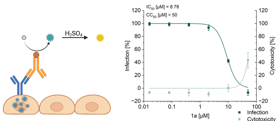
Figure 1: Schematic representation of the in-cell ELISA assay and the results for compound 1a.
